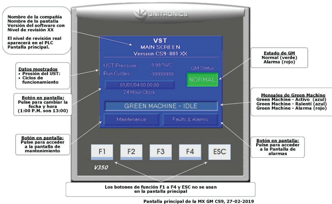
Figura 6-12: Pantalla principal
