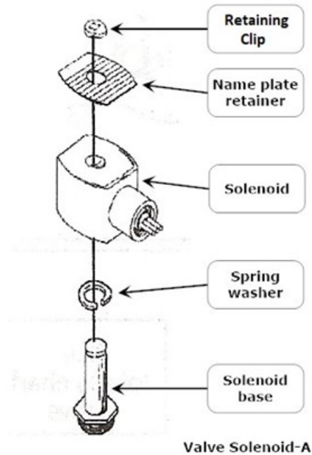
Valve Solenoid-A
