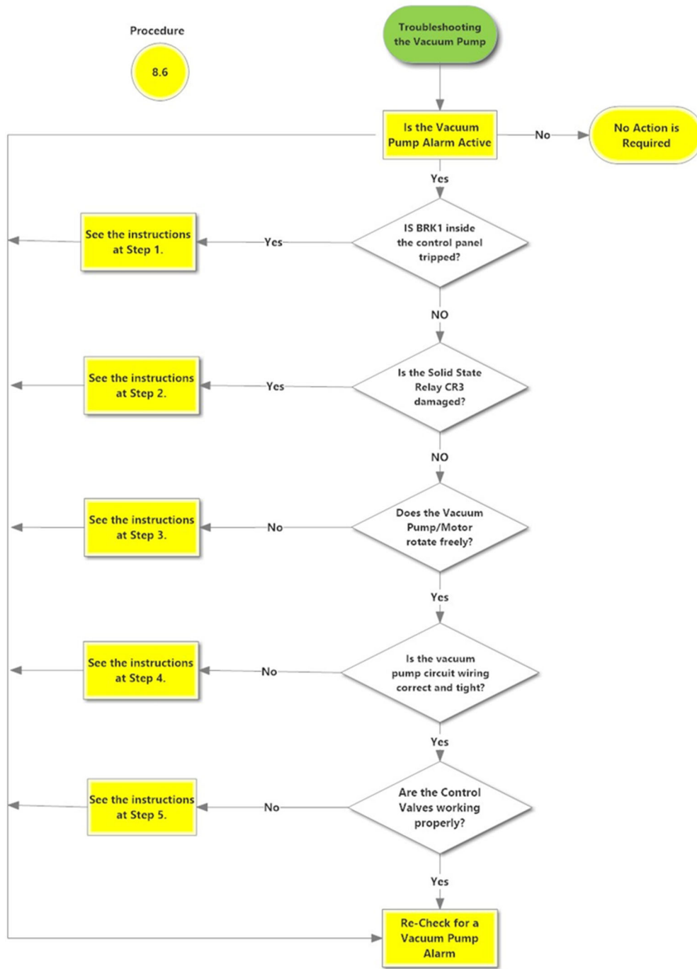
Vacuum Pump Motor Alarm, 10-6-2021
