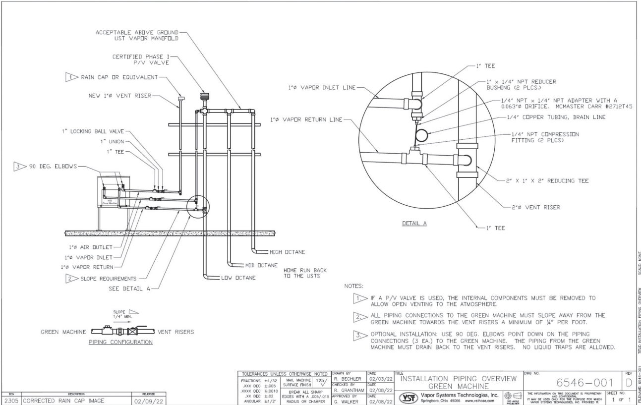
Figure 7-4: GREEN MACHINE Vapor Piping Layout
