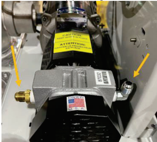
Figure 9-15: Two Tubes Removed from Vacuum Pump
