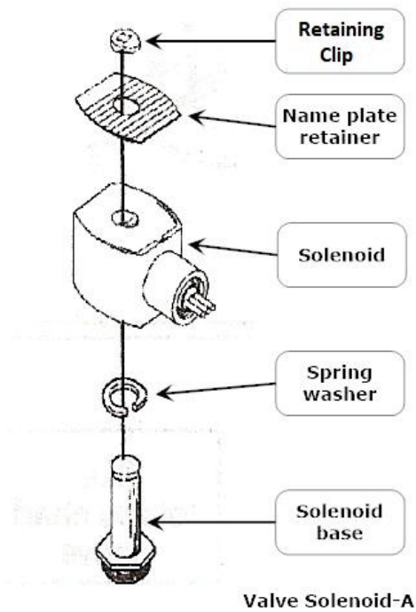
Figure 9-19: Valve Solenoid Assembly
