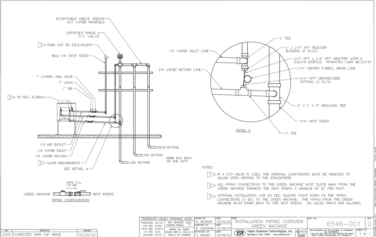
Figure 2-1: Vapor Piping Overview
