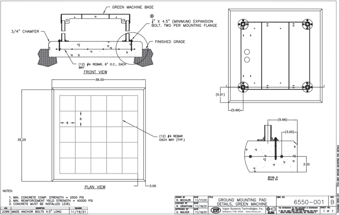
Figure 1-2: GREEN MACHINE Ground Mounting Pad
