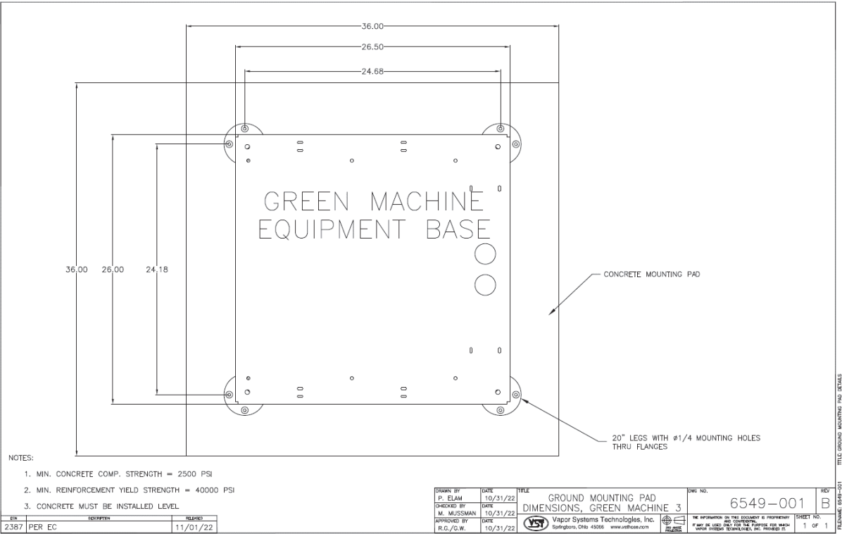
Figure 1-1: Concrete mounting pad dimensions
