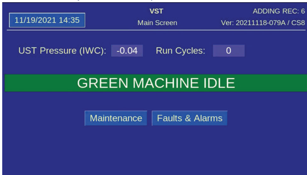
Figure 6-7: Pantalla principal
