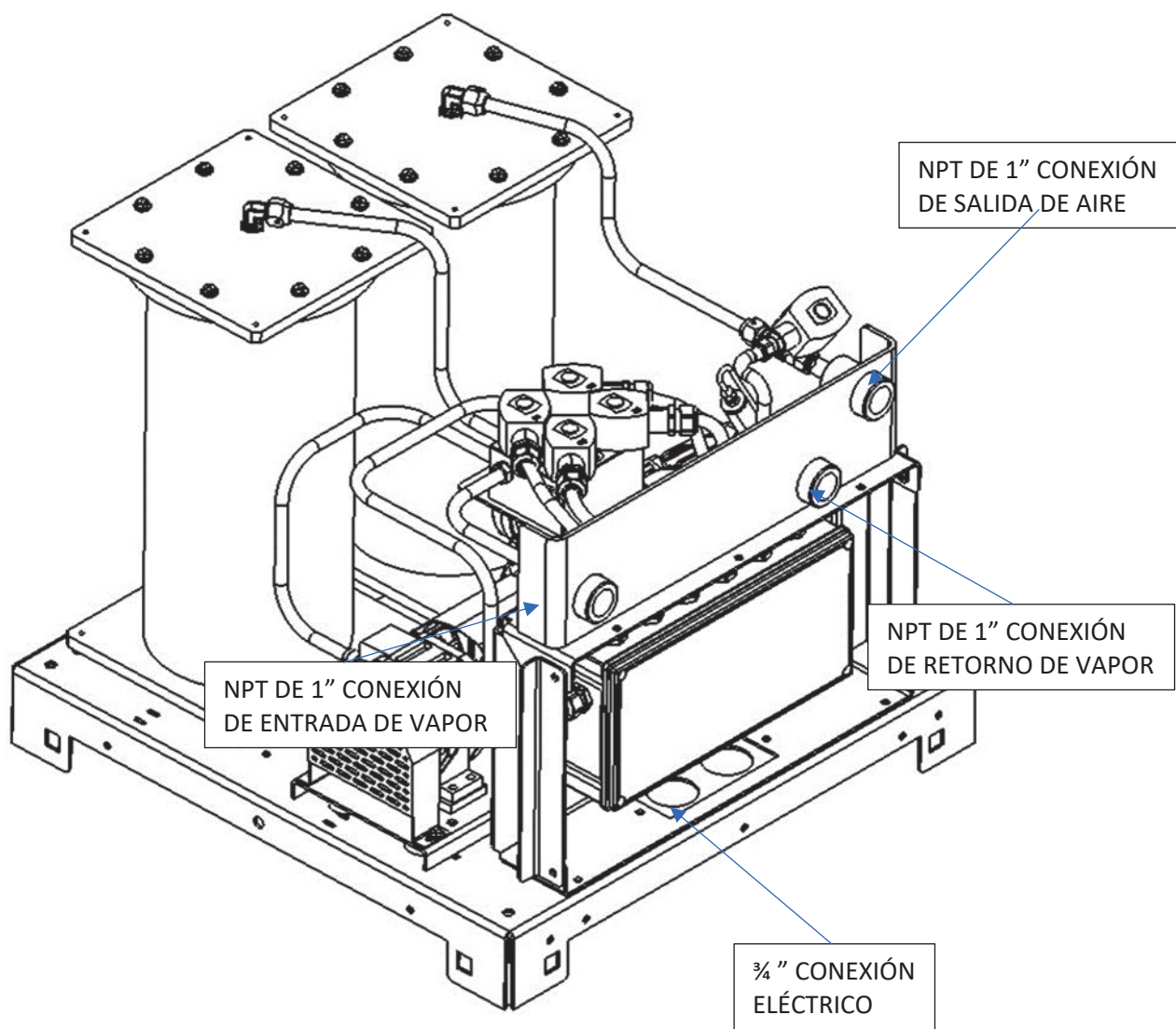
Figure 2-2: Conexiones de la GREEN MACHINE
