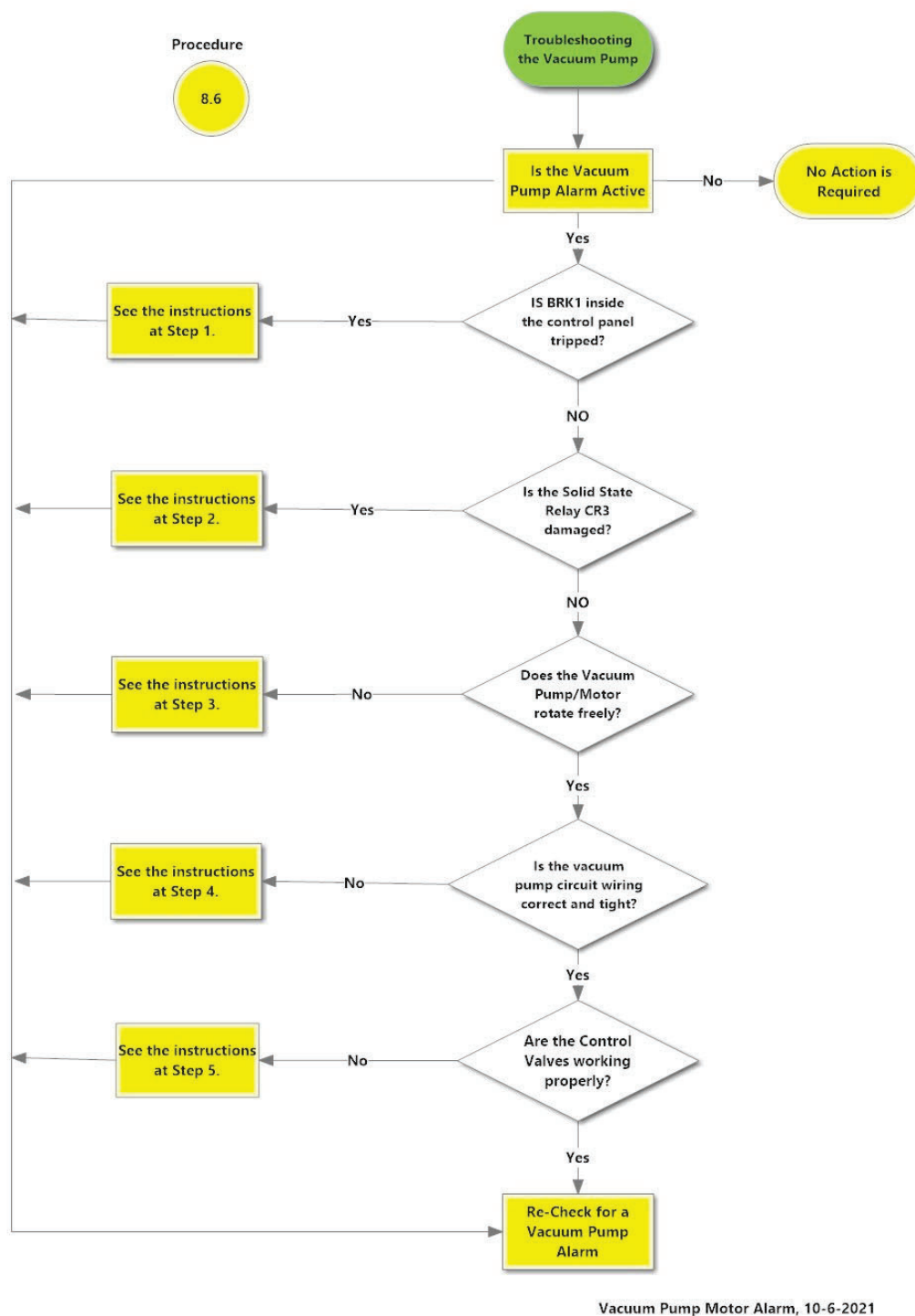
Figure 8-6: Vacuum Pump Troubleshooting Procedures
