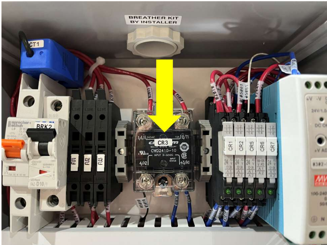
Figure 9-4: Vacuum Pump Solid State Relay
