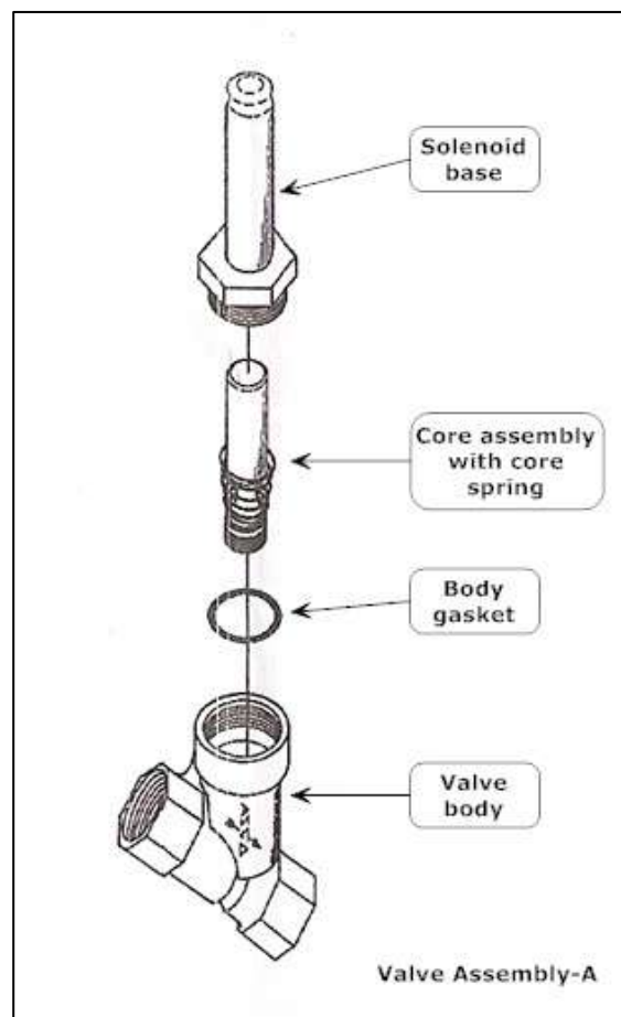
Figure 7-13: Valve Core Assembly
