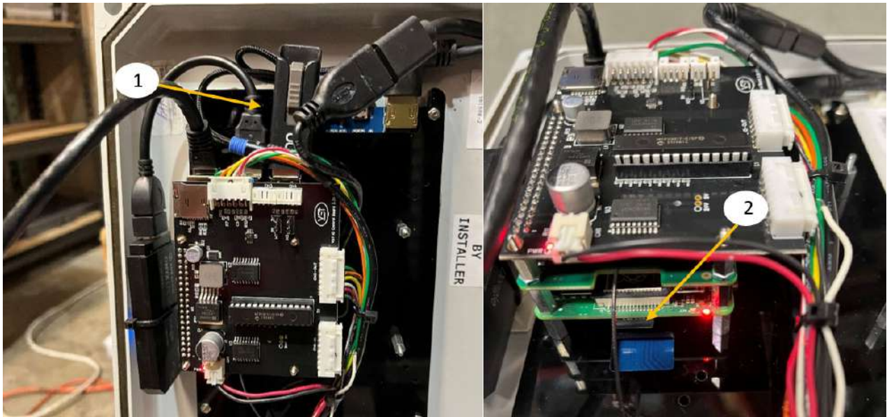
Figure 5-1: Primary and Secondary Data Storage Units
