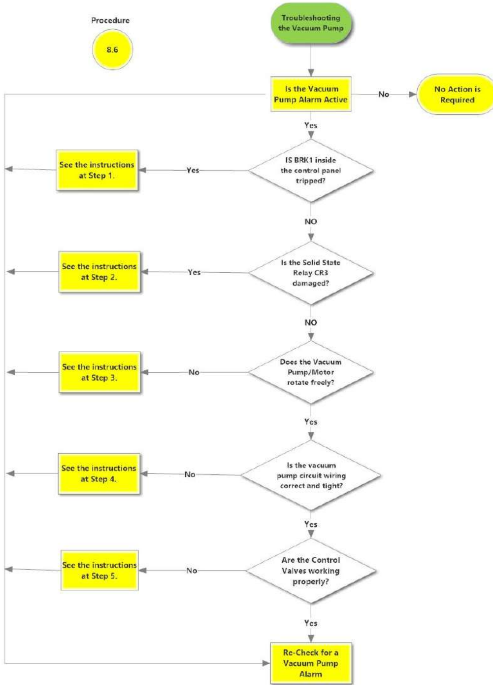
Figure 8-6: Vacuum Pump Troubleshooting Procedures
