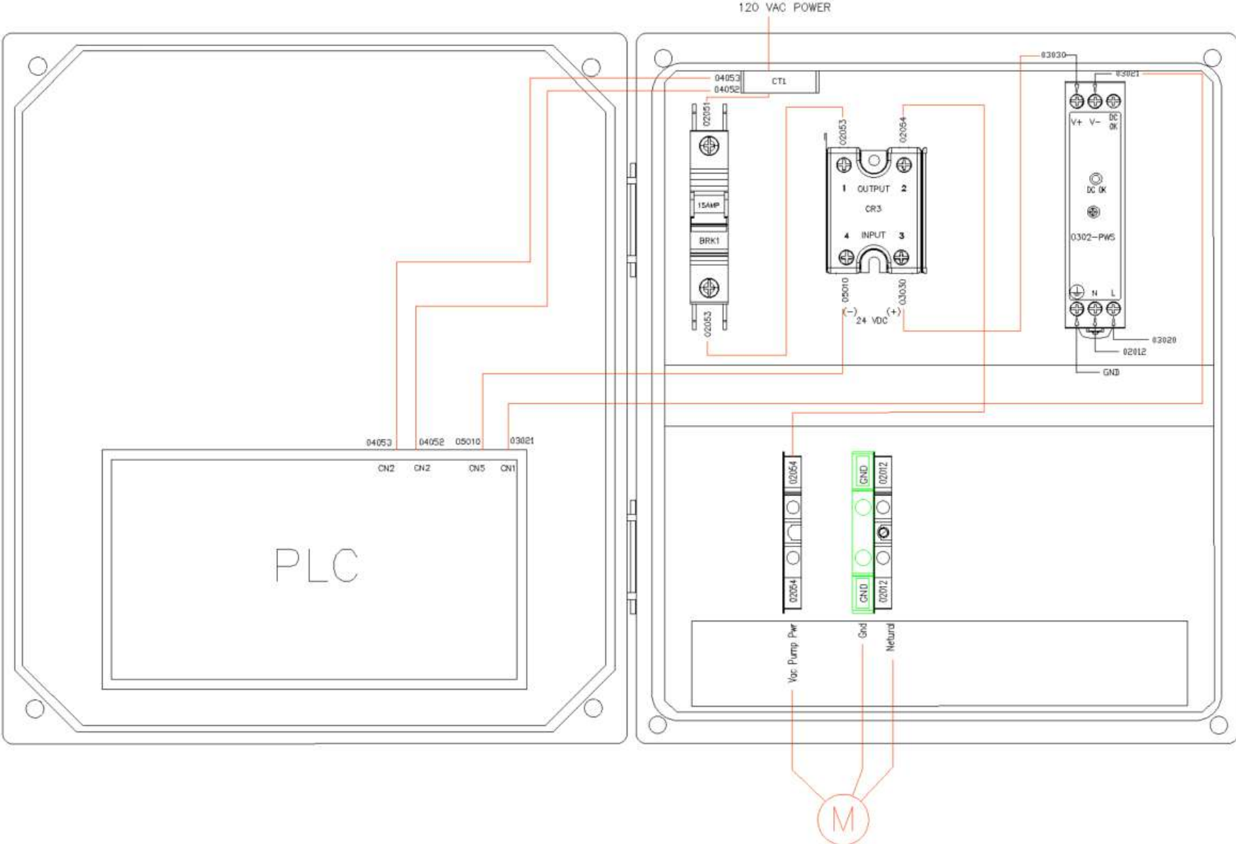
Figure 8-10: Vacuum Pump Circuit
