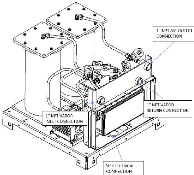
Figure 6-6: GREEN MACHINE Operation Diagram
