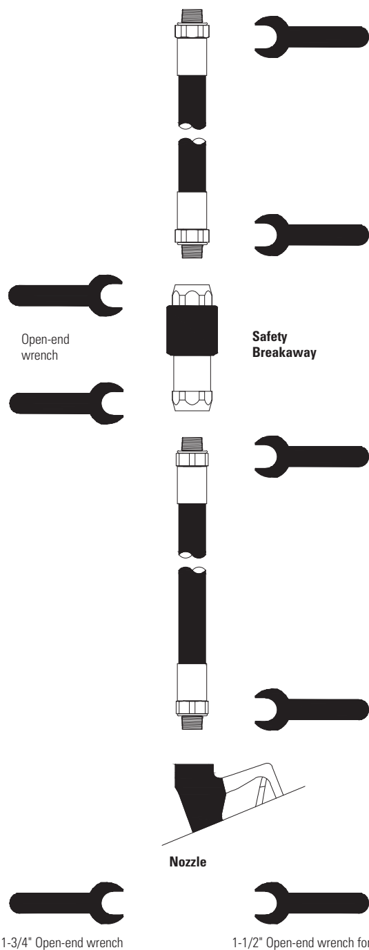
Figure 1. Hanging Hardware Assembly
