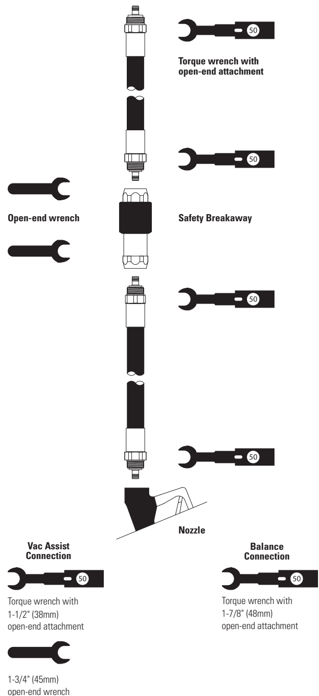
EVR Vacuum Assist Hanging Hardware Assembly
