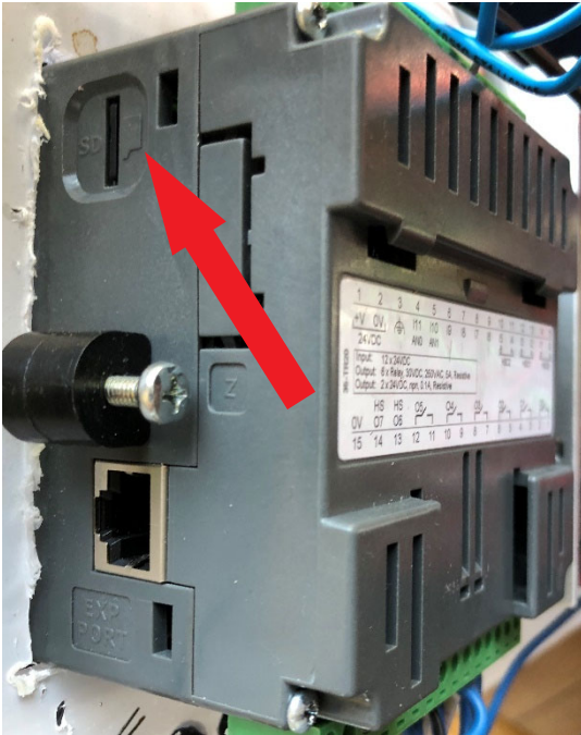
Figura: 5.7 Tarjeta microSD insertada
